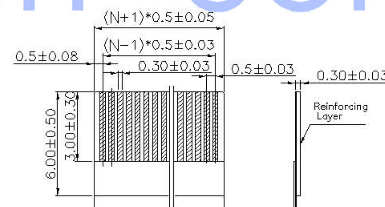
RECOMMENDED FFC/FPC DIM.
