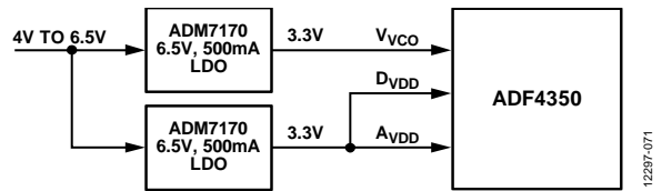
Figure 68. RF PLL/VCO Power
