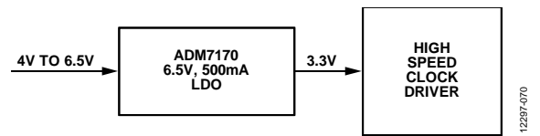
Figure 67. Clock Driver
