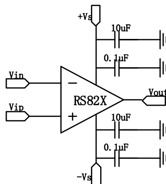
Figure1. Amplifier with Bypass Capacitors
