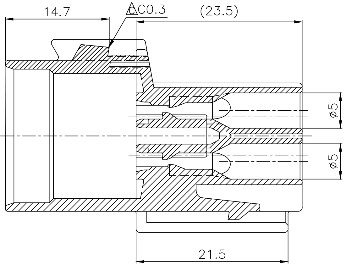
SECTION A-A(2/1)
