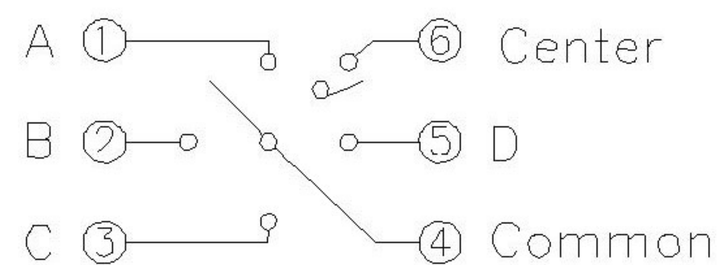
Circuit Diagram
