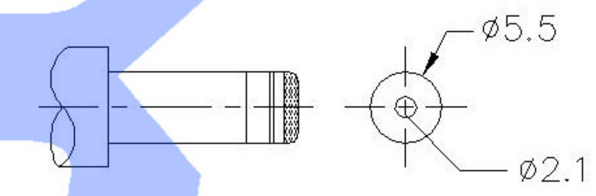
MATING PLUG Jack Insertion Depth: 9.15 mm
