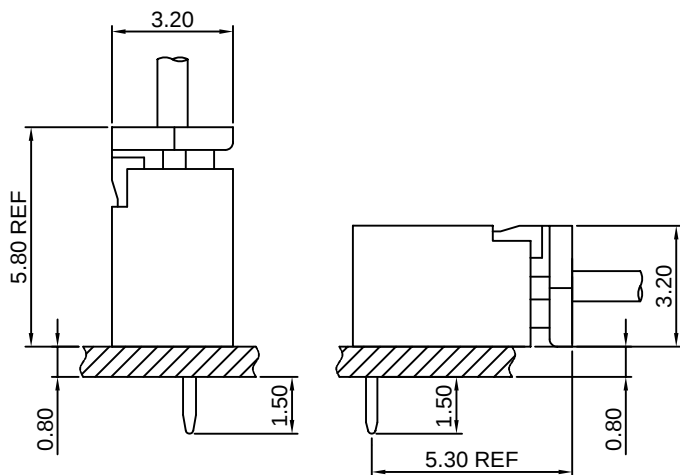
DIP YTPPE
