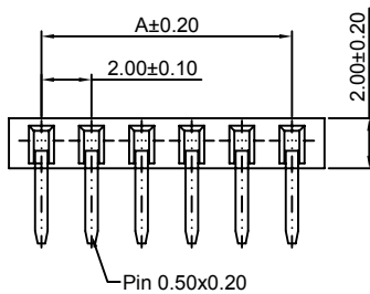
Pin 0.50x0.20
