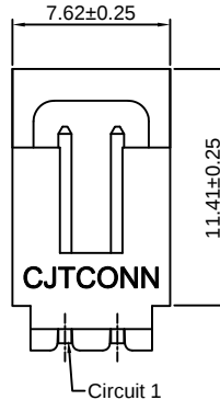
A2547WRD-2P(Black)
