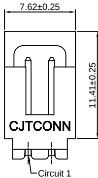
A2547WRC-2P(White)
