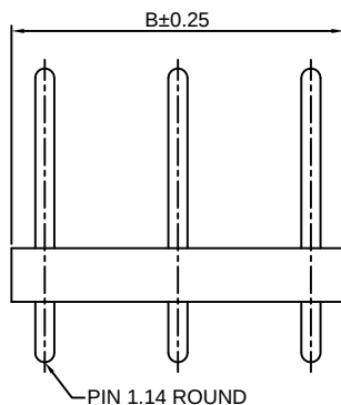
PIN 1.14 ROUND
