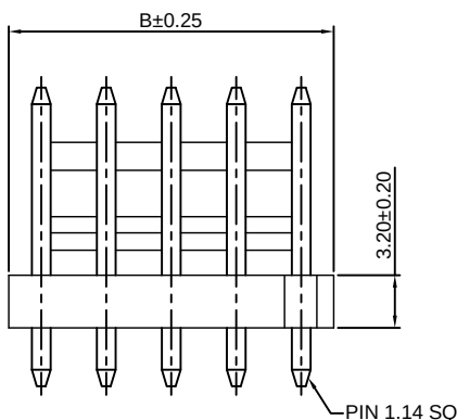
PIN 1.14 SQ
