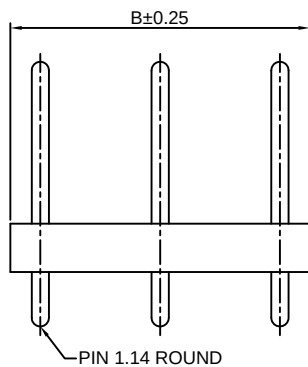
PIN 1.14 ROUND
