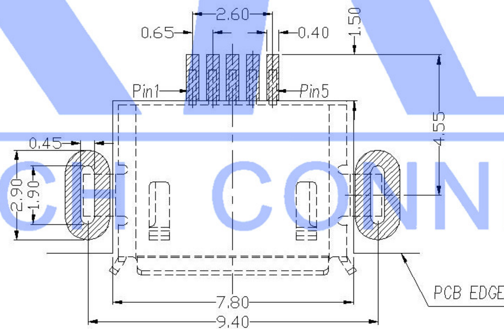
RECOMMENDED PCB LAYOUT
