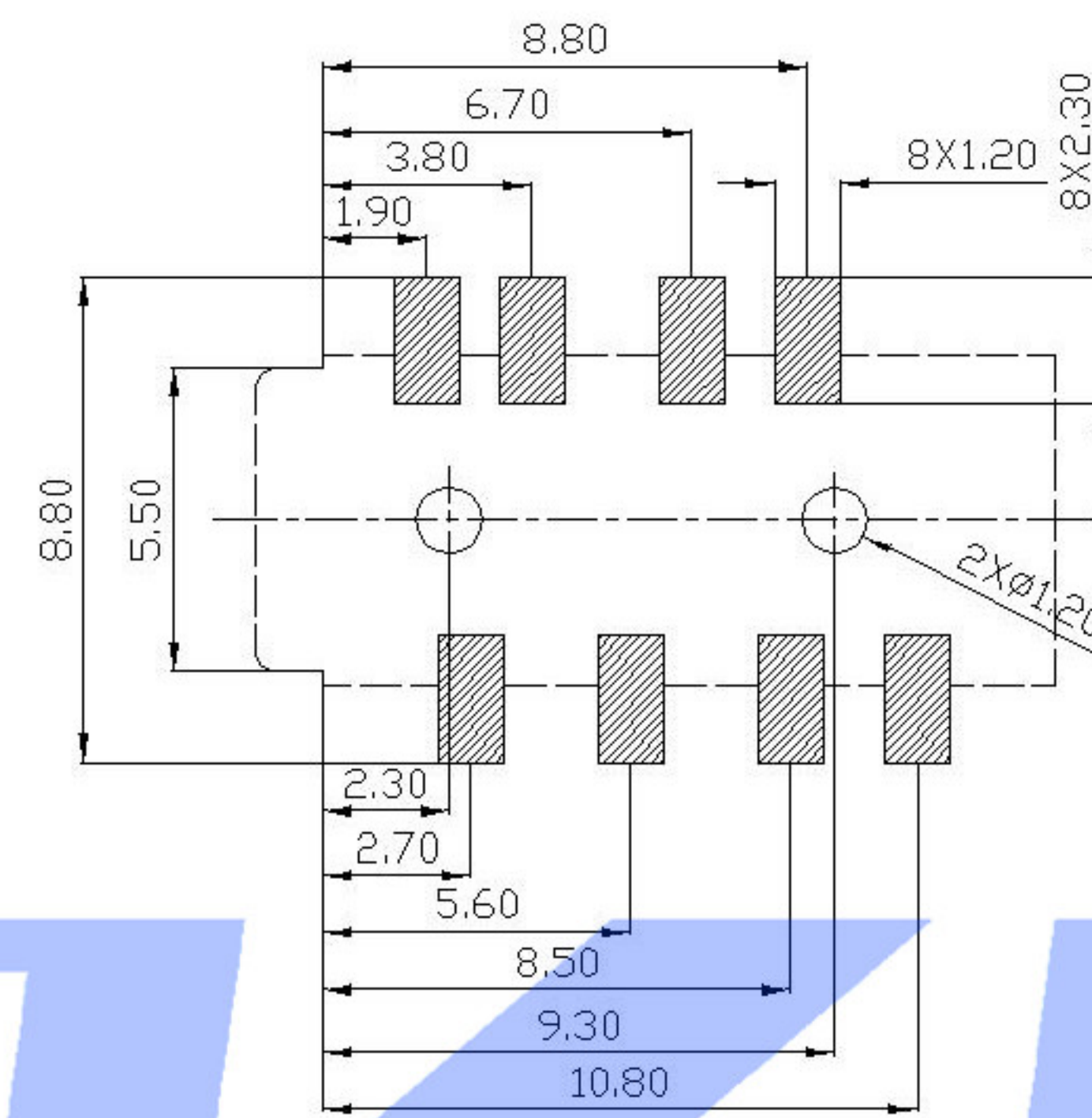
PCB LAYOUT TOP VIEW
