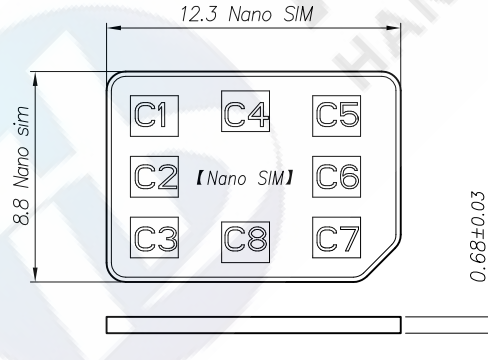
【 SIM Card Pin Assignments 】
