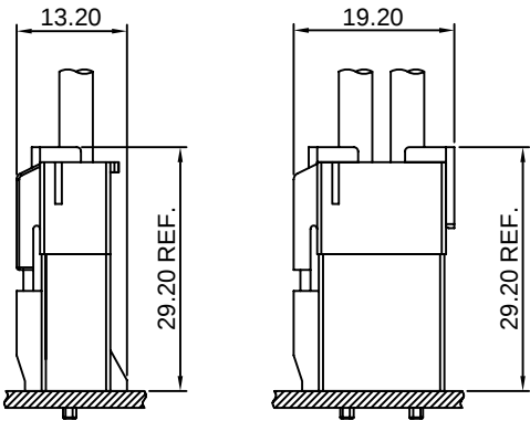
Inner-housing lock
