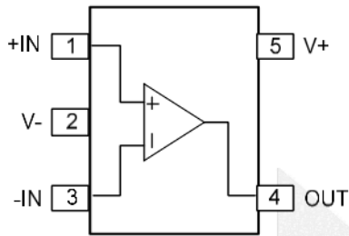
SC70-5
