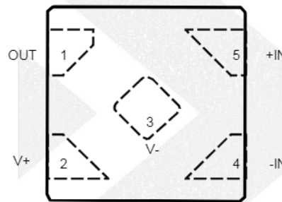
DFN0.8*0.8-4
