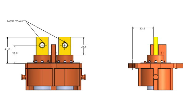
Busbar Type 1
