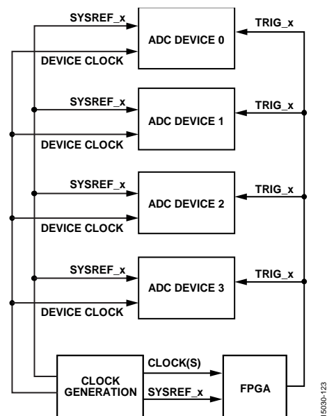
Figure 98. System Using TRIG x and SYSREF x for Synchronization
