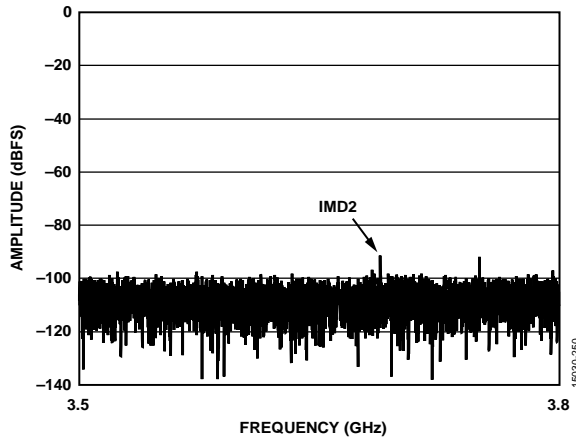
Figure 63. Two-Tone FFT, IMD2 Zoom In, f_{IN1} = 1841.5 MHz, f_{IN2} = 1846.5 MHz, A_{IN1} and A_{IN2} = -15 dBFS (see Figure 62), 10 GSFS
