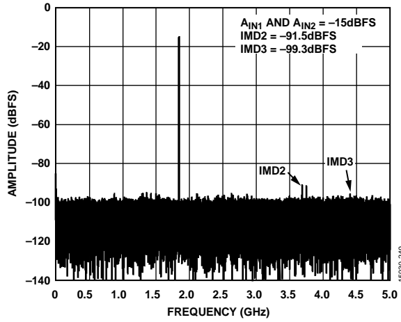
Figure 62. Two-Tone FFT, f_{IN1} = 1841.5 MHz, f_{IN2} = 1846.5 MHz, A_{IN1} and A_{IN2} = -15 dBFS, 10 GSFS
