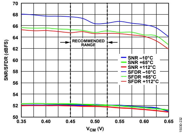
Figure 22. SNR/SFDR vs. V_{CM} , 6 GSPS
