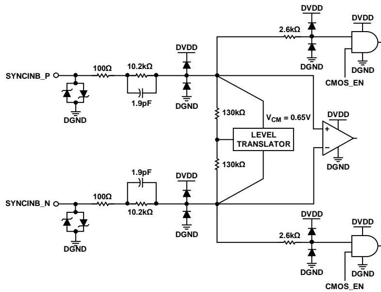
Figure 88. SYNCINB_x Inputs
