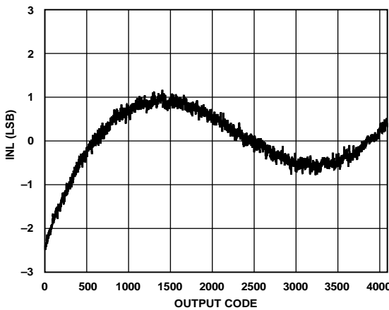
Figure 70. INL at f_{IN} = 170 MHz, 10 GSPS
