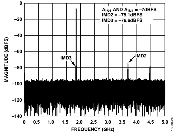
Figure 59. Two-Tone FFT, 10 GSPS, f_{IN1} = 1841.5 MHz, f_{IN2} = 1846.5 MHz, A_{IN1} and A_{IN2} = -7 dBFS
