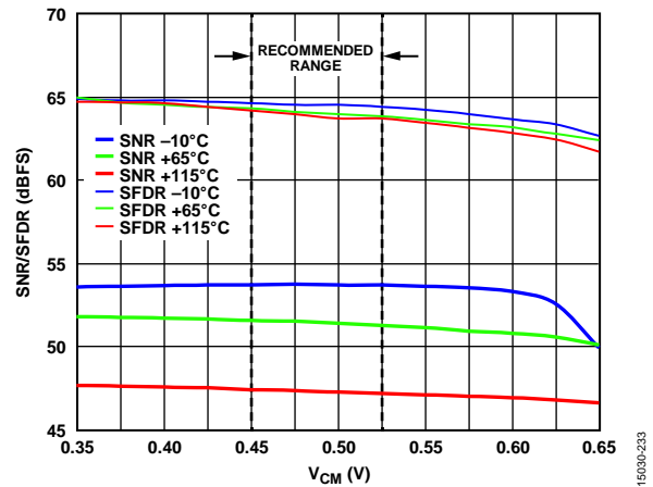
Figure 54. SNR/SFDR vs. V_{CM} , 10 GSPS
