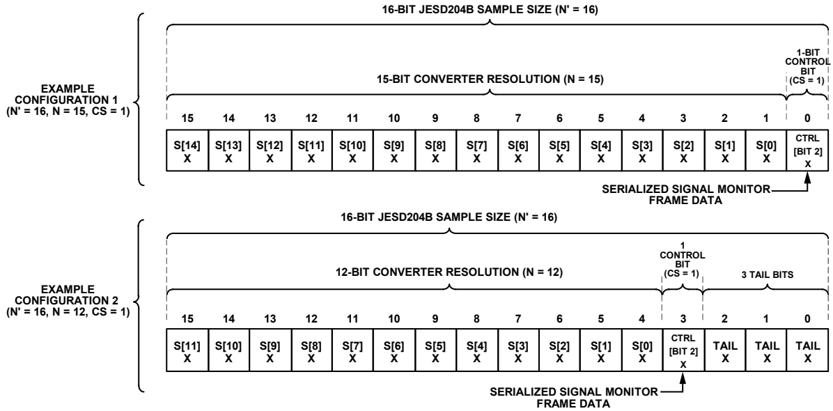
Figure 111. Signal Monitor Control Bit Location
