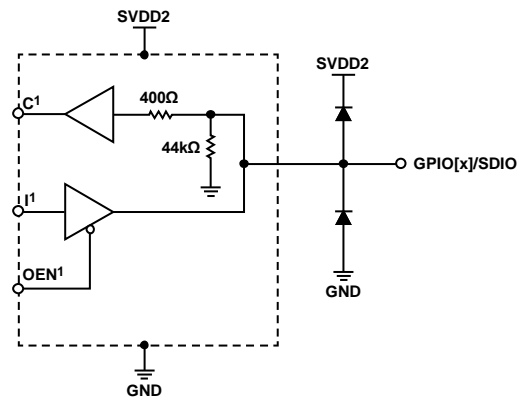
Figure 81. GPIO[x] and SDIO
