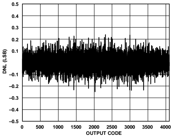
Figure 69. DNL at f_{IN} = 170 MHz, 10 GSPS
