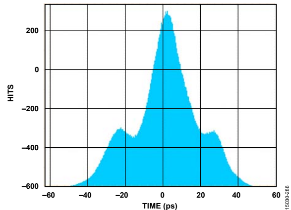
Figure 120. Digital Outputs Histogram, External 100 Ω Terminations at 16 Gbps
