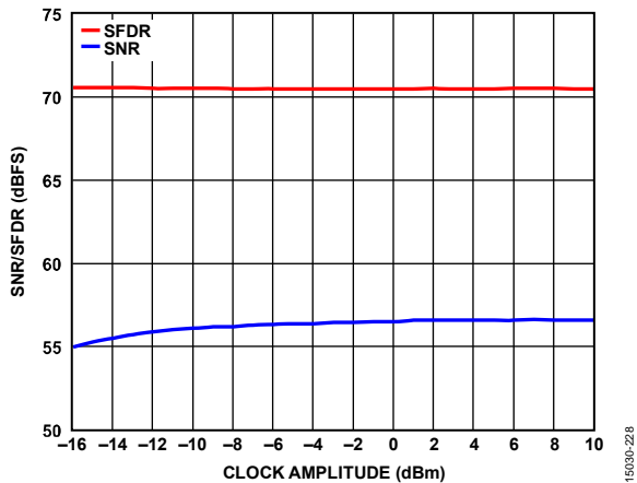
Figure 20. SNR/SFDR vs. Clock Amplitude at f_{IN} = 1000 MHz, 6 GSPS
