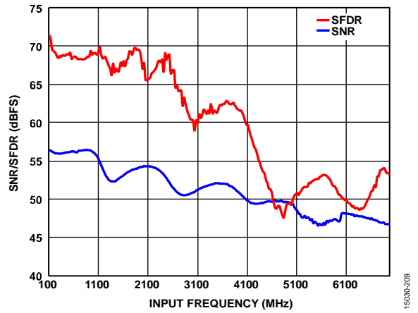
Figure 53. SNR/SFDR vs. Input Frequency ( f_{IN} ), A_{IN} = -1 dBFS
