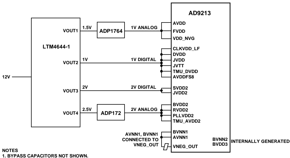
Figure 126. Alternate Simplified Power Supply Configuration
