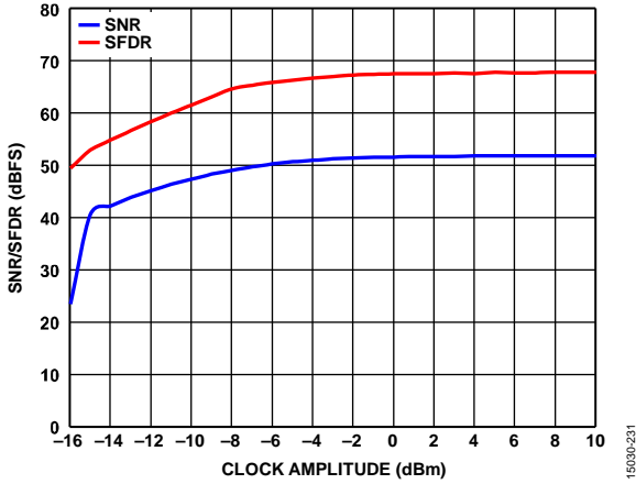
Figure 56. SNR/SFDR vs. Clock Amplitude, f_{IN} = 2600 MHz, 10 GSPS
