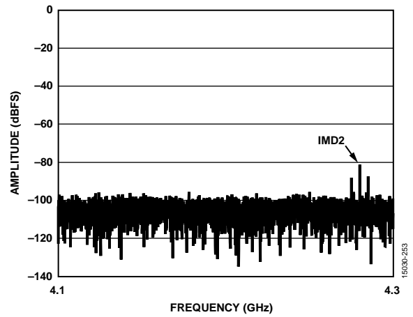
Figure 66. Two-Tone FFT, IMD2 Zoom In, f_{IN1} = 2137.5 MHz, f_{IN2} = 2142.5 MHz, A_{IN1} and A_{IN2} = -7 dBFS (see Figure 65), 10 GSFS
