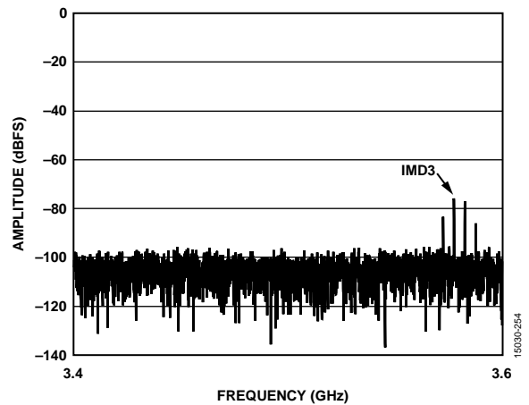
Figure 67. Two-Tone FFT, IMD3 Zoom In, f_{IN1} = 2137.5 MHz, f_{IN2} = 2142.5 MHz, A_{IN1} and A_{IN2} = -7 dBFS (see Figure 65), 10 GSFS
