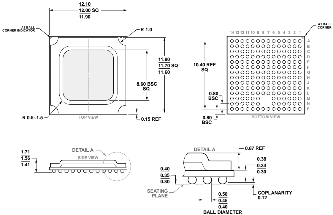
Figure 127. 192-Ball Ball Grid Array, Thermally Enhanced [BGA_ED] (BP-192-1) Dimensions shown in millimeters
