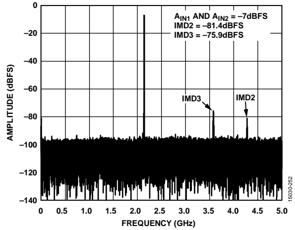
Figure 65. Two-Tone FFT, f_{IN1} = 2137.5 MHz, f_{IN2} = 2142.5 MHz, A_{IN1} and A_{IN2} = -7 dBFS, 10 GSFS
