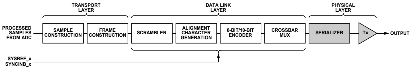
Figure 116. Data Flow
