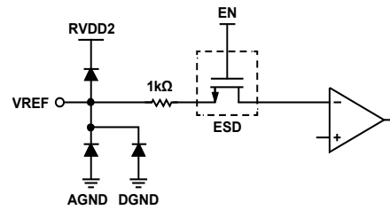
Figure 86. VREF
