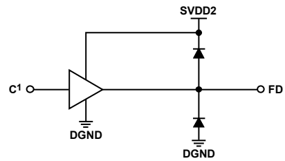
Figure 85. FD
