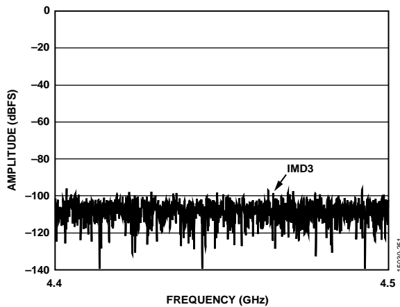
Figure 64. Two-Tone FFT, IMD3 Zoom In, f_{IN1} = 1841.5 MHz, f_{IN2} = 1846.5 MHz, A_{IN1} and A_{IN2} = -15 dBFS (see Figure 62), 10 GSFS
