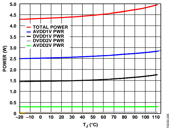
Figure 58. Power vs. T_j , f_{IN} = 2600 MHz, 10 GSPS
