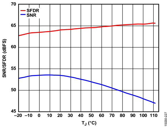
Figure 57. SNR/SFDR vs. T_j , f_{IN} = 2600 MHz, 10 GSPS
