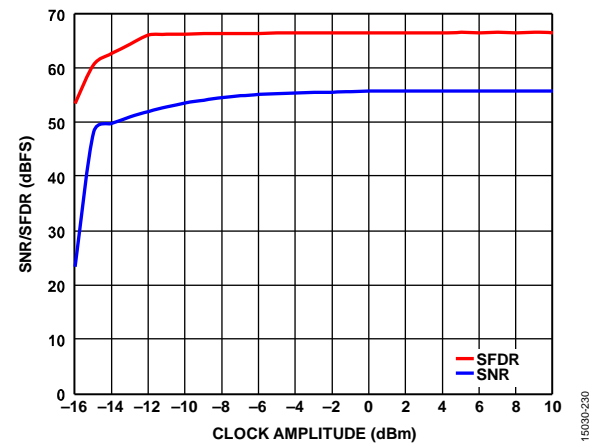
Figure 55. SNR/SFDR vs. Clock Amplitude, f_{IN} = 1000 MHz, 10 GSPS
