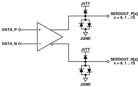
Figure 76. Digital Outputs
