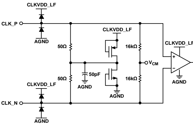
Figure 78. Clock Inputs
