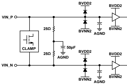
Figure 77. Analog Inputs
