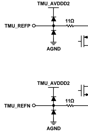
Figure 79. TMU_REFx Inputs
