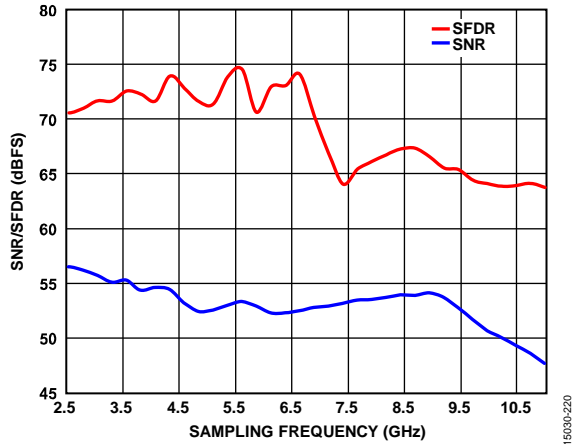
Figure 50. SNR/SFDR vs. Sampling Frequency, f_{IN} = 2600 MHz, 10 GSPS
