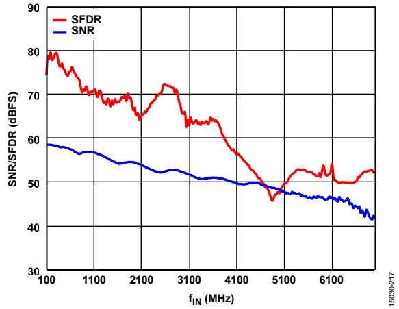
Figure 19. SNR/SFDR vs. f_{IN} , A_{IN} = -1 dBFS, 6 GSPS
