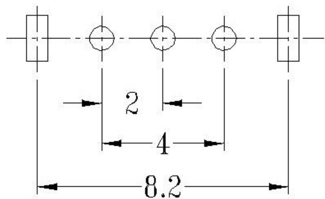
P.C.B. LAYOUT BOTTOM VIEW
