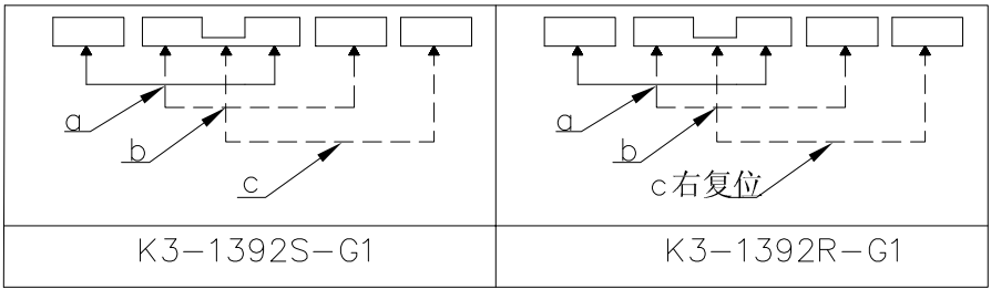
Schematic(Shorting)
