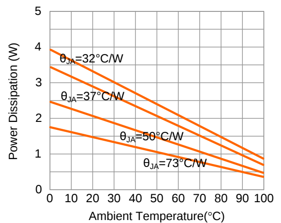
Maximum Power Dissipation(TO-263)
