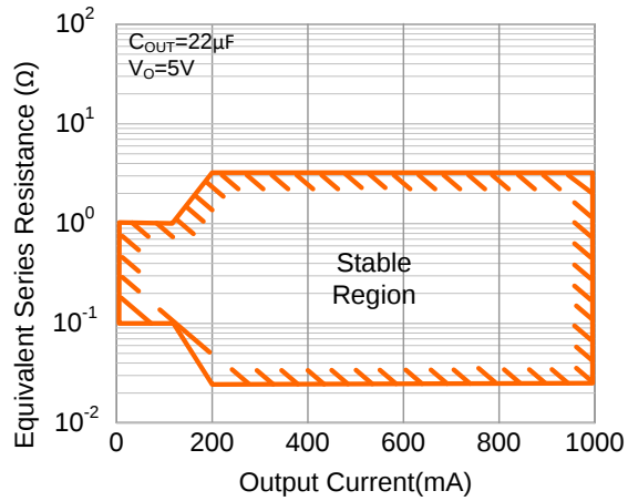
Output Capacitor ESR
