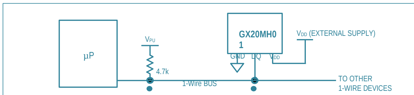
Figure 5. Powering the GX20MH01 with an External Supply
