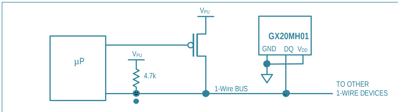
Figure 4. Supplying the Parasite-Powered GX20MH01 During Temperature Conversions
