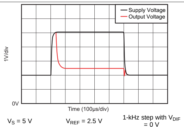
Figure 22. Brownout Recovery
