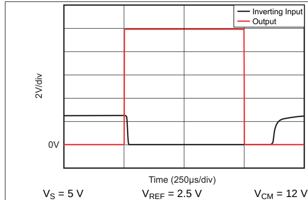
Figure 19. Inverting Differential Input Overload
