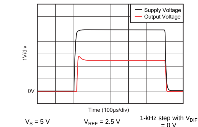
Figure 21. Start-Up Response
