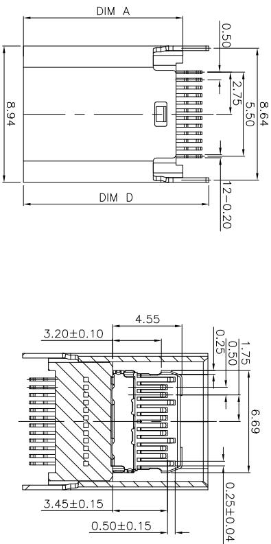
SECTION B-B SCALE 1:1
