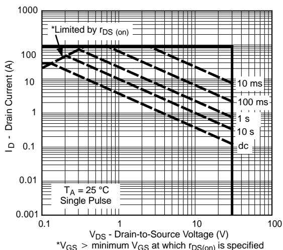
* V_{GS} > minimum V_{GS} at which r_{DS(on)} is specified Safe Operating Area, Junction-to-Ambient
