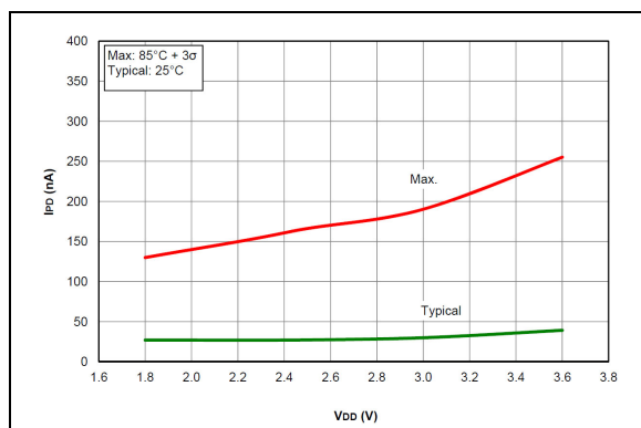
FIGURE 36-13: IPD BASE, Low-Power Sleep Mode, PIC16LF18313/18323 Only
