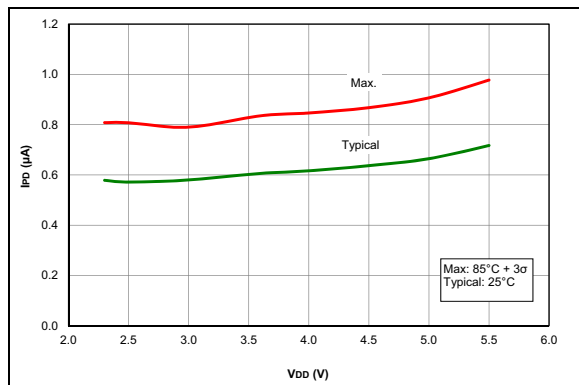
FIGURE 36-15: IPD, Watchdog Timer (WDT), PIC16F18313/18323 Only
