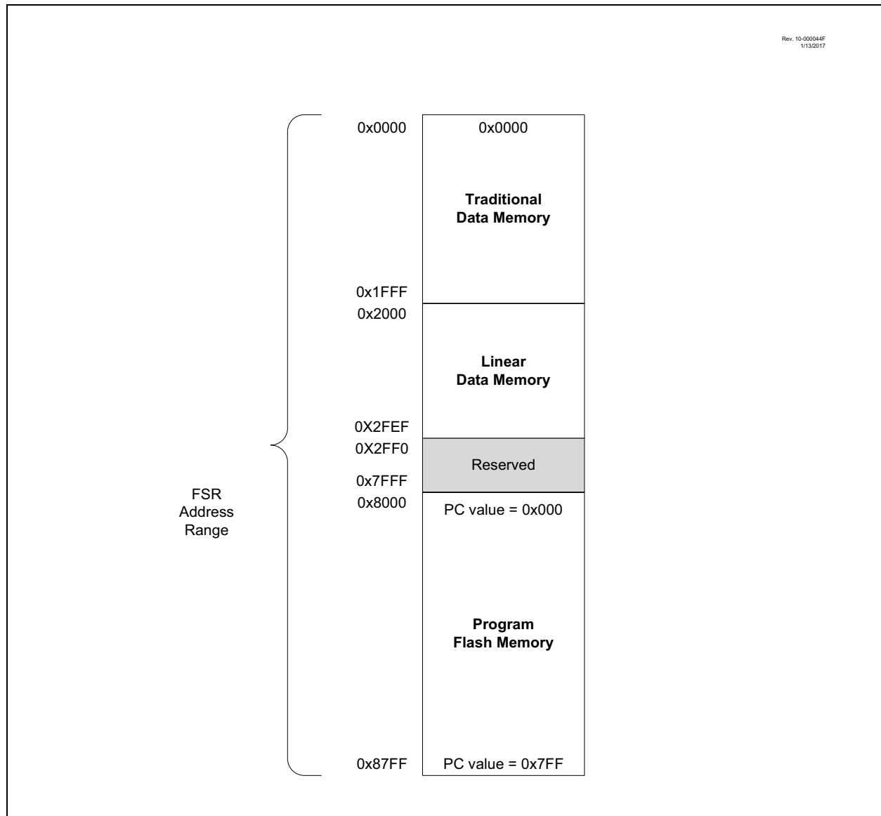
FIGURE 4-8: INDIRECT ADDRESSING
