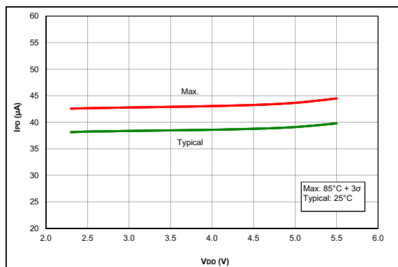
FIGURE 36-17: IPD, Fixed Voltage Reference (FVR), PIC16F18313/18323 Only
