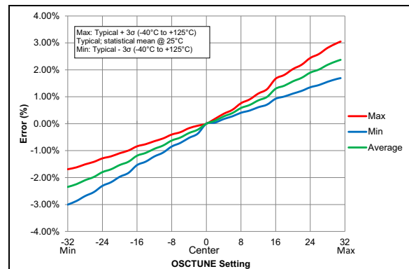
FIGURE 36-108: OSCUNE Center Frequency
