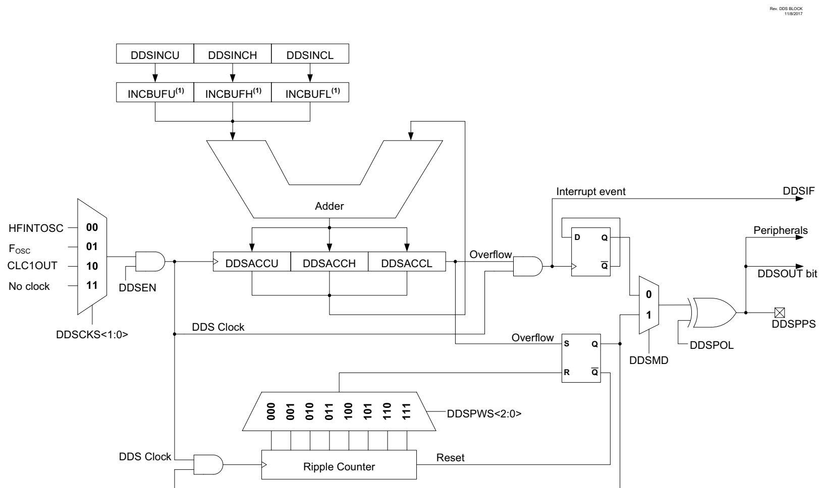
FIGURE 23-1: NUMERICALLY CONTROLLED OSCILLATOR MODULE SIMPLIFIED BLOCK DIAGRAM
