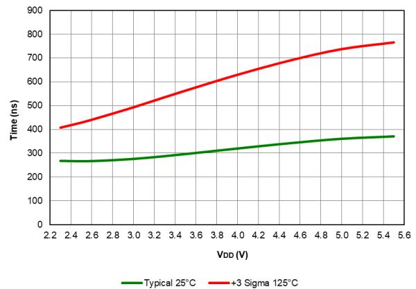
Figure 41-90. FVR Stabilization Period, PIC16LF18424/44 only
