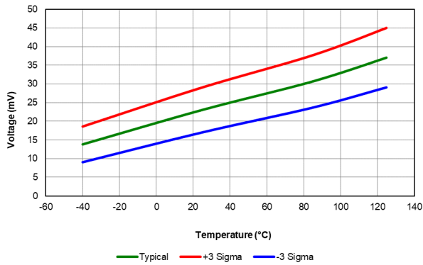
Figure 41-45. LPBOR Reset Hysteresis, All devices
