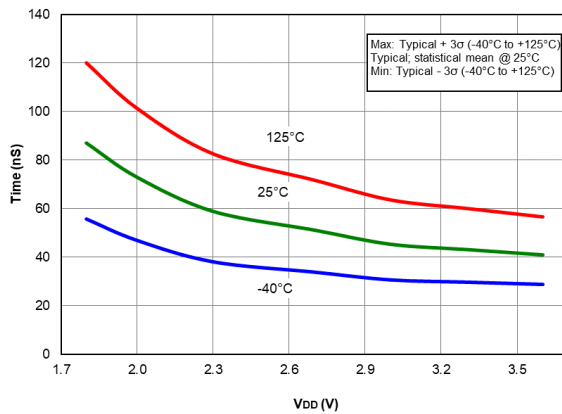
Figure 41-85. Comparator Response Time Falling Edge, PIC16LF18424/44 only
