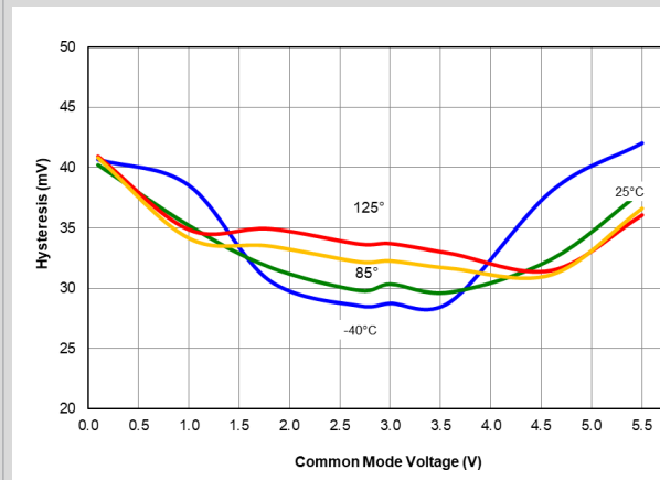
Figure 41-80. Comparator Hysteresis, Normal Power Mode ( CxSP = 1 ), V_{DD} = 5.5V , Typical Measured Values, PIC16F18424/44 only
