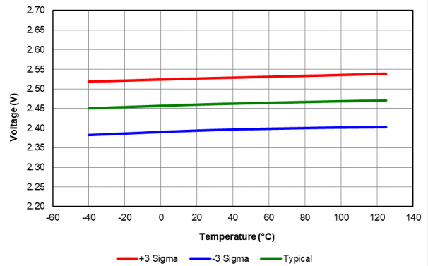
Figure 41-44. LPBOR Reset Voltage, All devices
