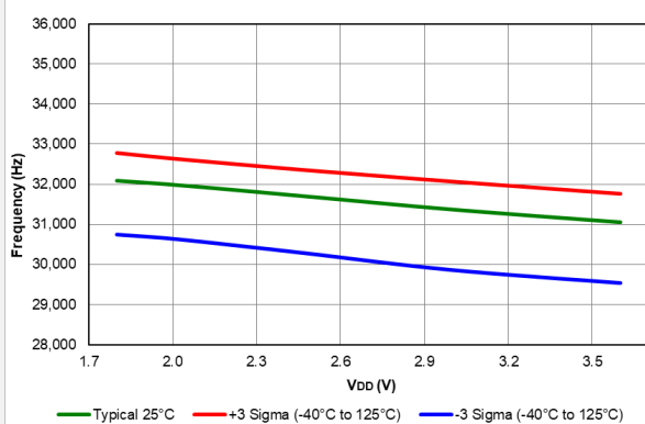
Figure 41-25. LFINTOSC Frequency, PIC16LF18424/44 only
