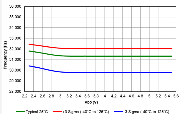
Figure 41-26. LFINTOSC Frequency, PIC16F18424/44 only
