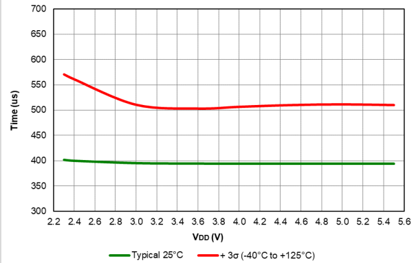
Figure 41-112. Wake from Sleep, VREGPM = 1, PIC16F18424/44 only
