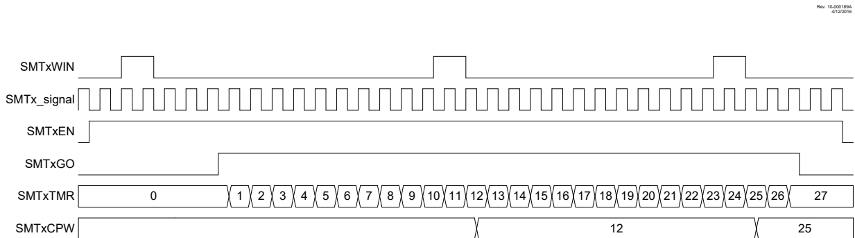
Figure 21-17. Counter Mode Timing Diagram
