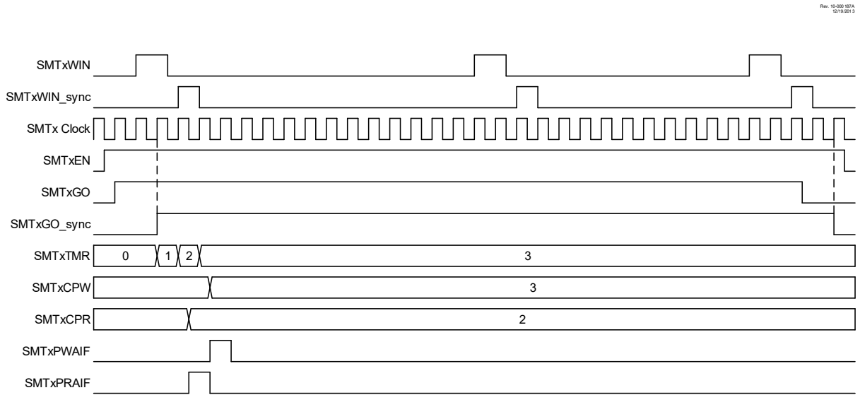
Figure 21-16. Capture Mode, Single Acquisition Timing Diagram
