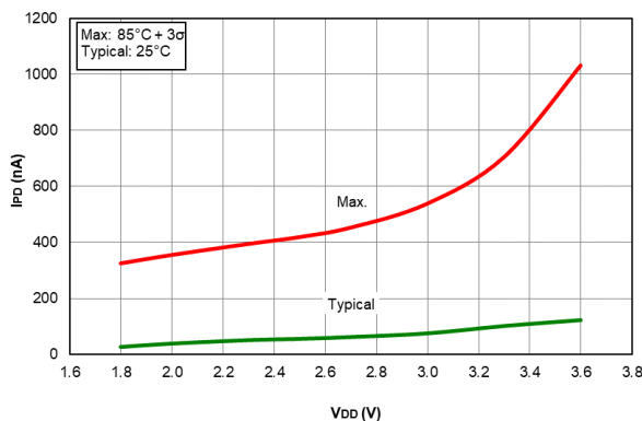
Figure 41-1. I_{PD} Base, Low-Power Sleep Mode PIC16LF18424/44 only
