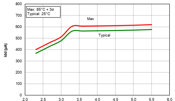
Figure 41-14. I_{DD} XT Oscillator 4 MHz, PIC16F18424/44 only
