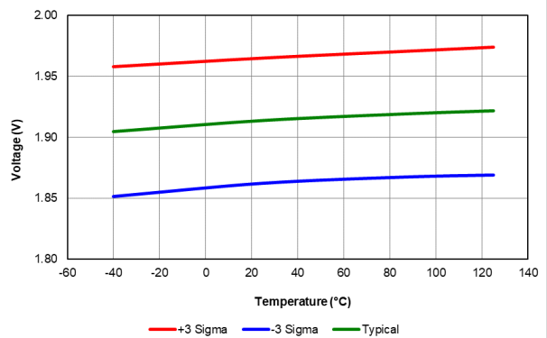
Figure 41-42. Brown-Out Reset Voltage, Trip Point BORV = 01, PIC16F18424/44 only
