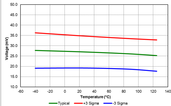
Figure 41-43. Brown-Out Reset Hysteresis, Trip Point BORV = 01, PIC16F18424/44 only
