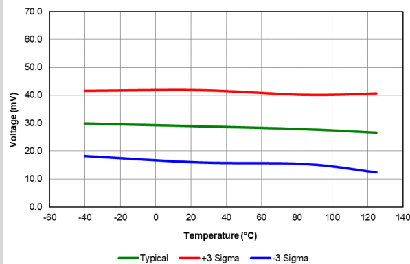
Figure 41-41. Brown-Out Reset Hysteresis, Trip Point BORV = 01, PIC16LF18424/44 only
