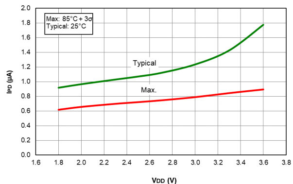
Figure 41-2. I_{PD} Watchdog Timer (WDT) PIC16LF18424/44 only
