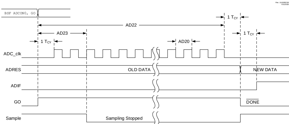
Figure 40-10. ADC Conversion Timing (ADC Clock F_{OSC} -Based)
