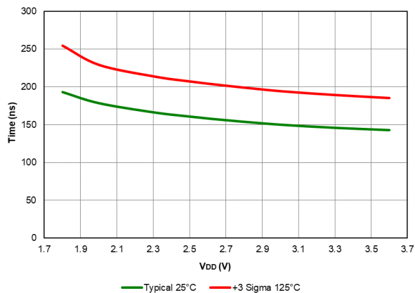
Figure 41-85. Comparator Response Time Falling Edge, PIC16LF18424/44 only
