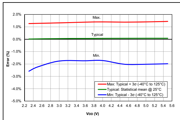
FIGURE 36-27: HFINTOSC Typical Frequency Error, PIC16F18313/18323 Only
