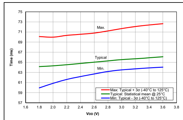
FIGURE 36-108: PWRT Period, PIC16LF18313/18323 Only
