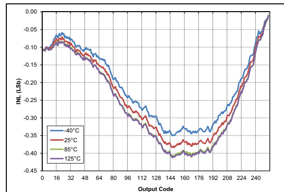
FIGURE 36-72: Typical DAC INL Error, V_{DD} = 5.0\text{V} , V_{REF} = \text{External } 5\text{V} , PIC16F18313/18323 Only
