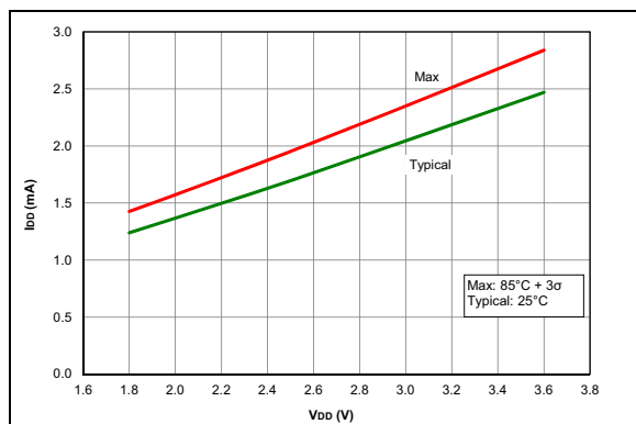
FIGURE 36-5: I_{DD} , HFINTOSC Mode, F_{OSC} = 32 MHz, PIC16LF18313/18323 Only
