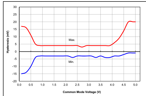
FIGURE 36-82: Comparator Offset, Normal Power Mode ( CxSP = 1 ), V_{DD} = 5.0V , Typical Measured Values at 25°C, PIC16F18313/18323 Only
