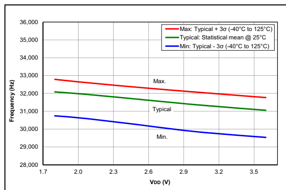
FIGURE 36-29: LFINTOSC Frequency, PIC16LF18313/18323 Only
