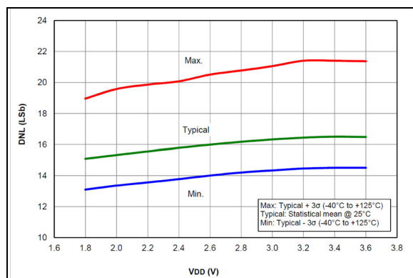
FIGURE 36-73: DAC INL Error, V_{DD} = 3.0V , PIC16LF18313/18323 Only
