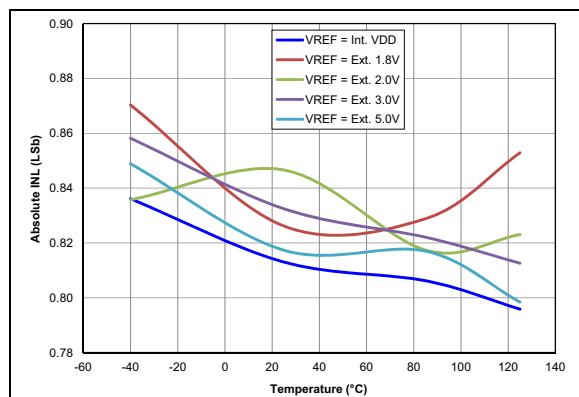
FIGURE 36-77: Absolute Value of DAC INL Error, V_{DD} = 5.0V , V_{REF} = V_{DD} , PIC16F18313/18323 Only
