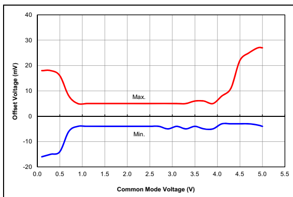
FIGURE 36-83: Comparator Offset, Normal Power Mode ( CxSP = 1 ), V_{DD} = 5.5V , Typical Measured Values from -40°C to 125°C, PIC16F18313/18323 Only
