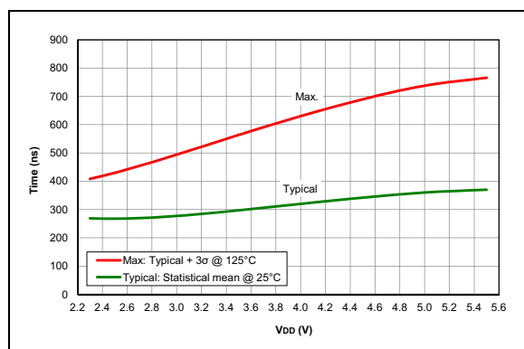
FIGURE 36-89: Comparator Response Time Rising edge, PIC16F18313/18323 Only
