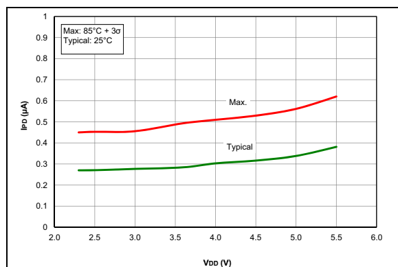
FIGURE 36-25: IPD BASE, 11, PIC16F18313/18323 Only
