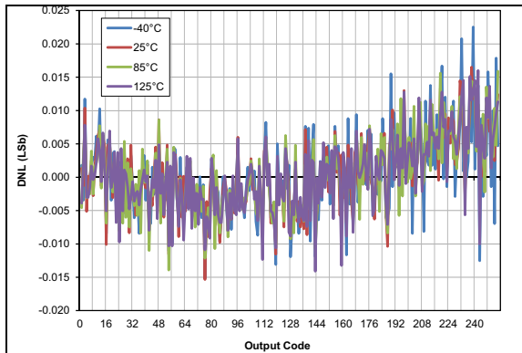
FIGURE 36-69: Typical DAC DNL Error, V_{DD} = 3.0\text{V} , V_{REF} = \text{External } 3\text{V} , All devices
