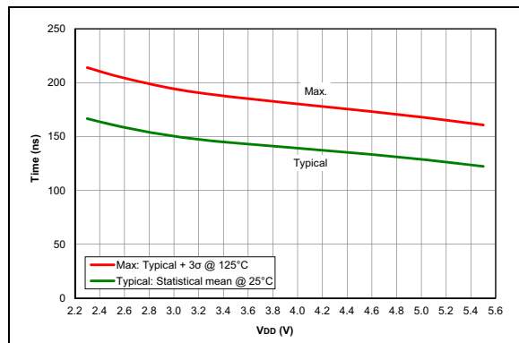
FIGURE 36-87: Comparator Response Time Falling edge, PIC16F18313/18323 Only
