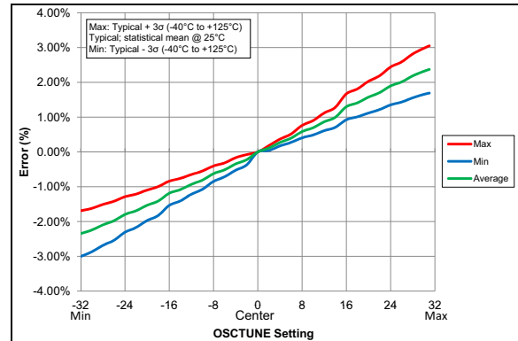
FIGURE 36-104: OSCUNE Center Frequency, PIC16LF18313/18323 Only
