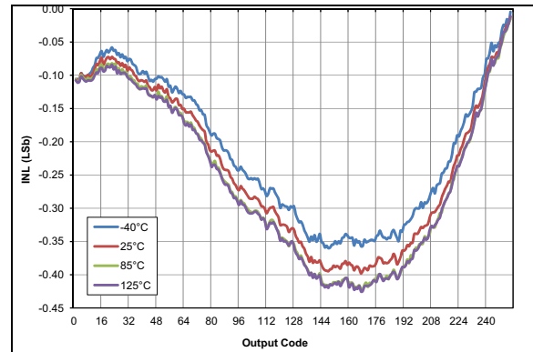
FIGURE 36-70: Typical DAC INL Error, V_{DD} = 3.0\text{V} , V_{REF} = \text{External } 3\text{V} , All devices
