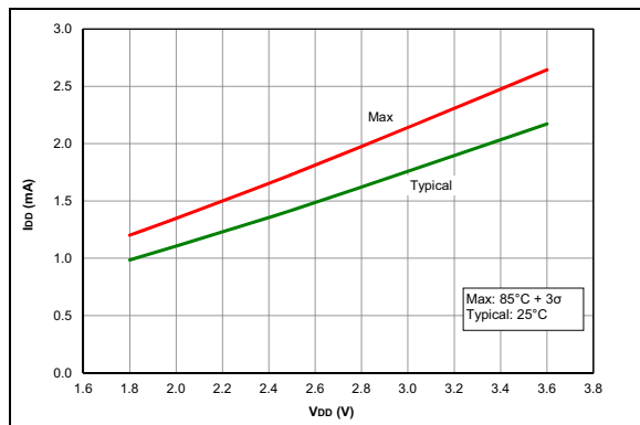
FIGURE 36-3: I_{DD} , HS Oscillator, 32 MHz, PIC16LF18313/18323 Only
