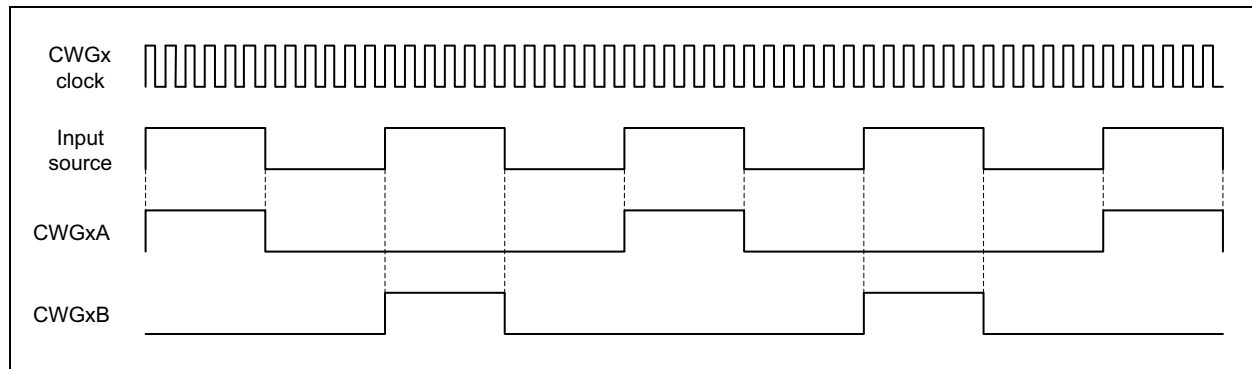
FIGURE 20-2: CWG1 PUSH-PULL MODE OPERATION
