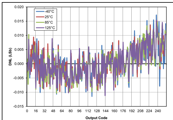
FIGURE 36-71: Typical DAC DNL Error, V_{DD} = 5.0\text{V} , V_{REF} = \text{External } 5\text{V} , PIC16F18313/18323 Only
