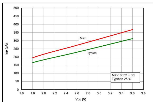
FIGURE 36-1: I_{DD} , XT Oscillator, 4 MHz, PIC16LF18313/18323 Only
