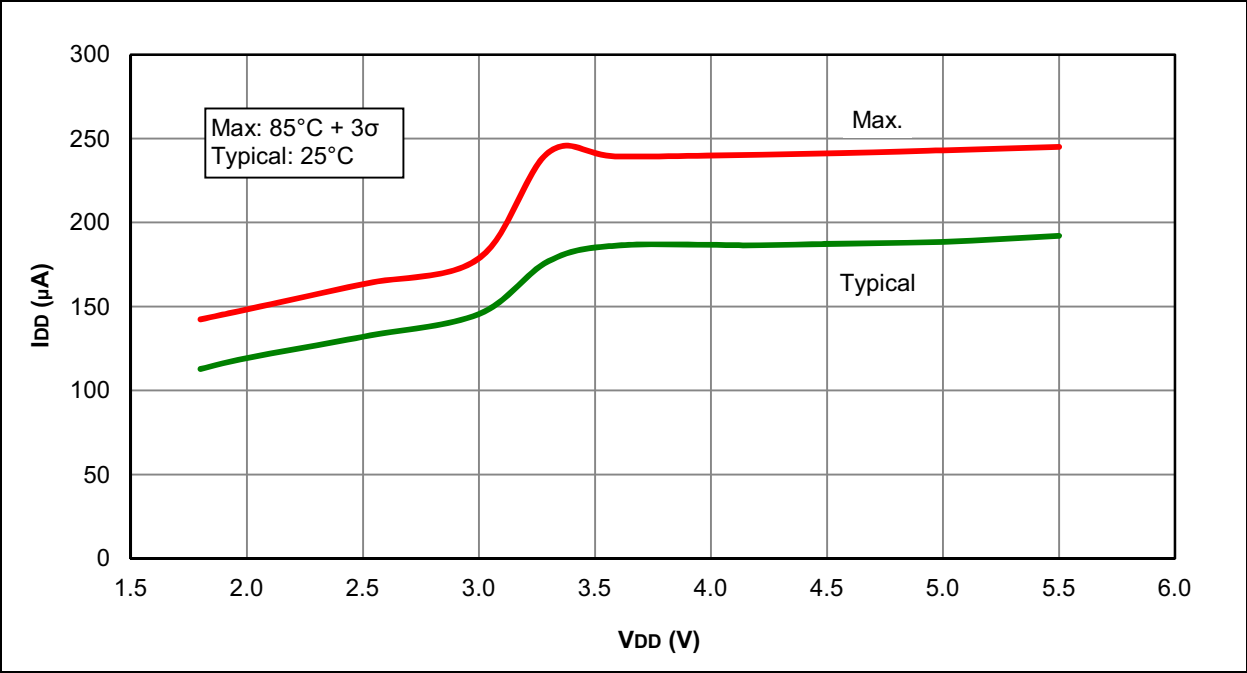
FIGURE 31-22: I DD , MFINTOSC, F osc = 500 kHz, PIC16F1938/9 ONLY
