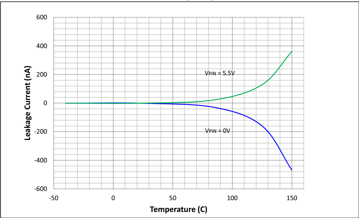
FIGURE 33-20: TYPICAL I IL vs. TEMPERATURE (MCLR)
