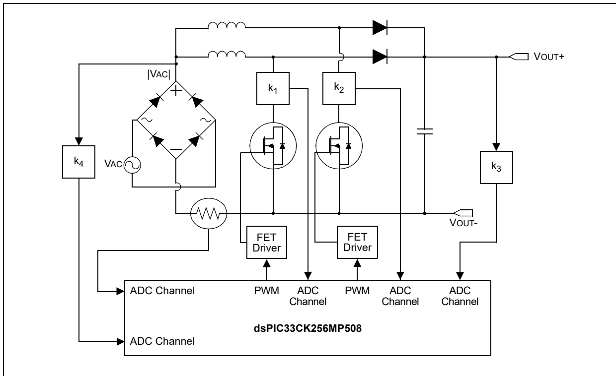
FIGURE 2-4: INTERLEAVED PFC
