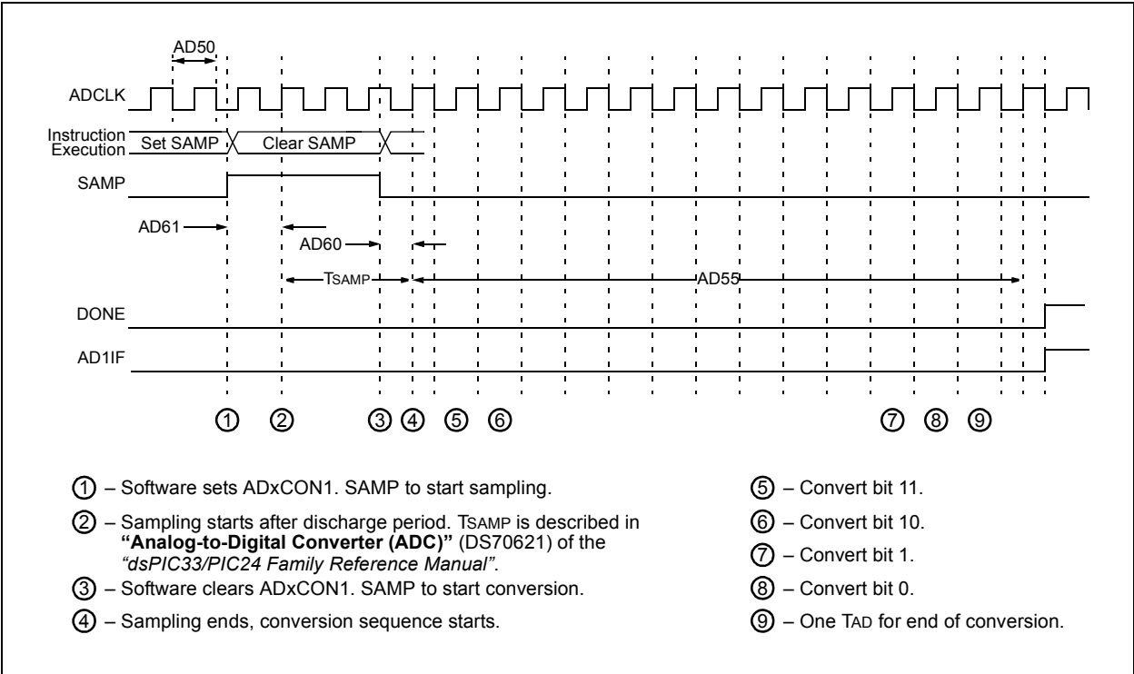
FIGURE 30-34: ADC CONVERSION (12-BIT MODE) TIMING CHARACTERISTICS (ASAM = 0, SSR[2:0] = 000, SSRCG = 0)
