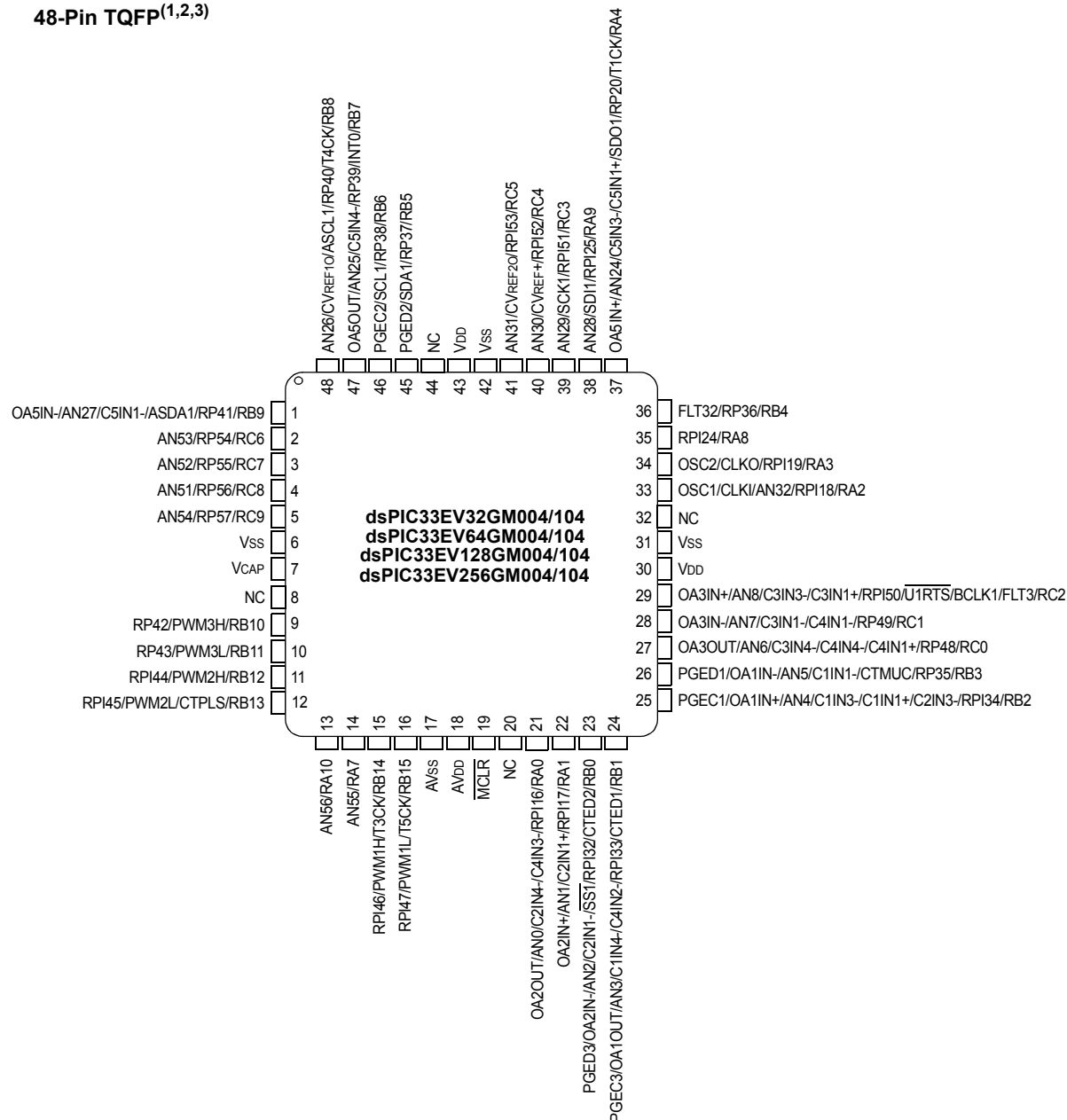
48-Pin TQFP (1,2,3)
