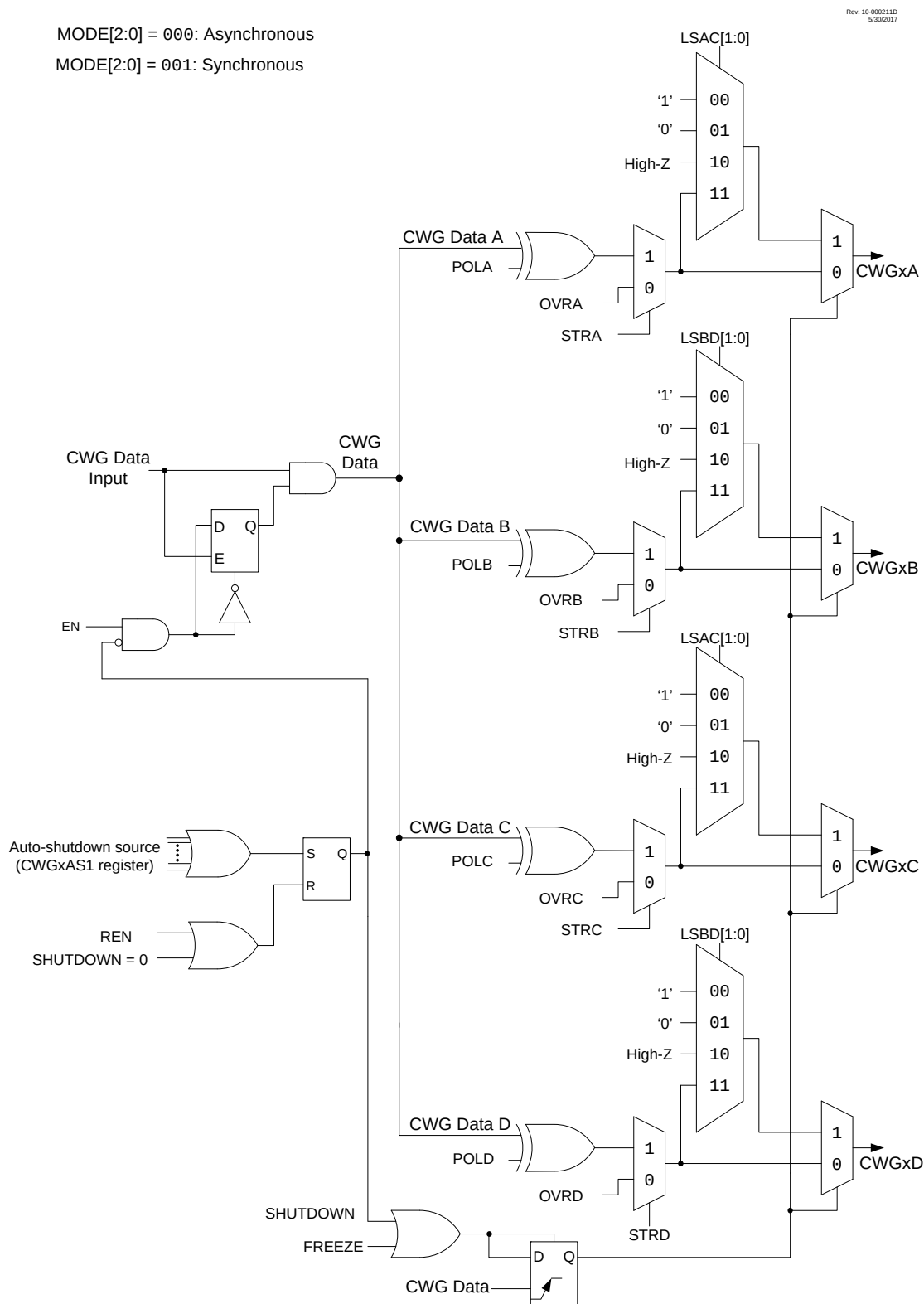
Figure 24-9. Simplified CWG Block Diagram (Output Steering Modes)
