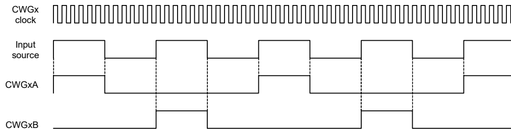
Figure 24-10. Example of Synchronous Steering ( MODE = 001)
