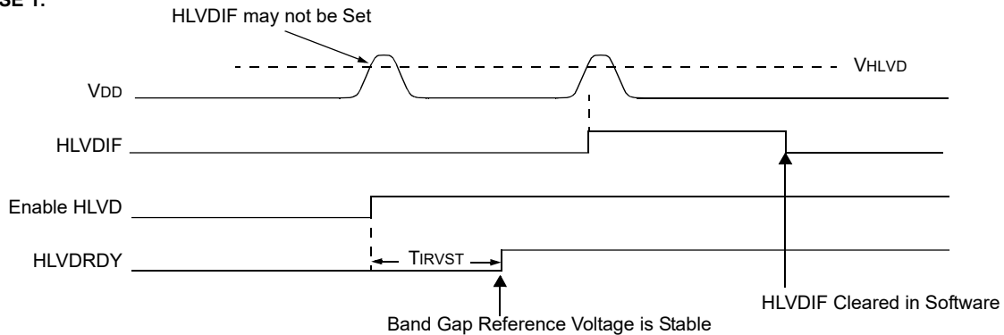
Figure 34-3. High-Voltage Detect Operation (INTH = 1)
