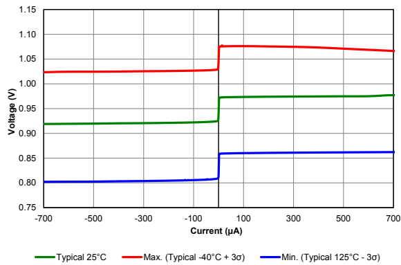
Figure 40-86. ZCD Behavior, V DD = 5.5V
