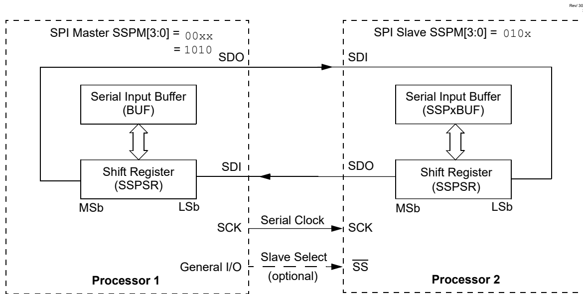
Figure 27-3. SPI Master/Slave Connection
