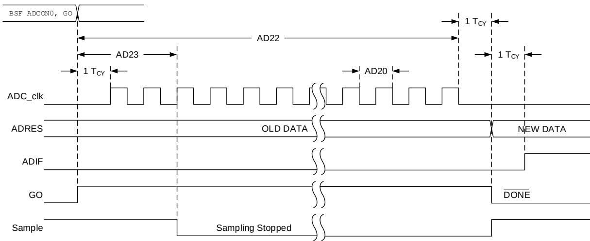
Figure 39-9. ADC Conversion Timing (ADC Clock F OSC -Based)
