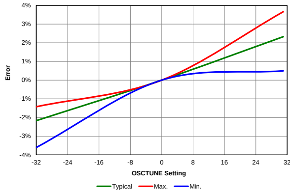
Figure 40-63. OSCTUNE Frequency Range (Normalized to Center Frequency)
