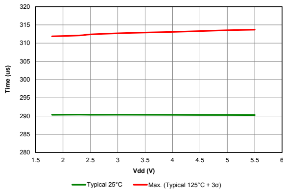
Figure 40-56. Wake From Sleep, VREGPM = 'b01
