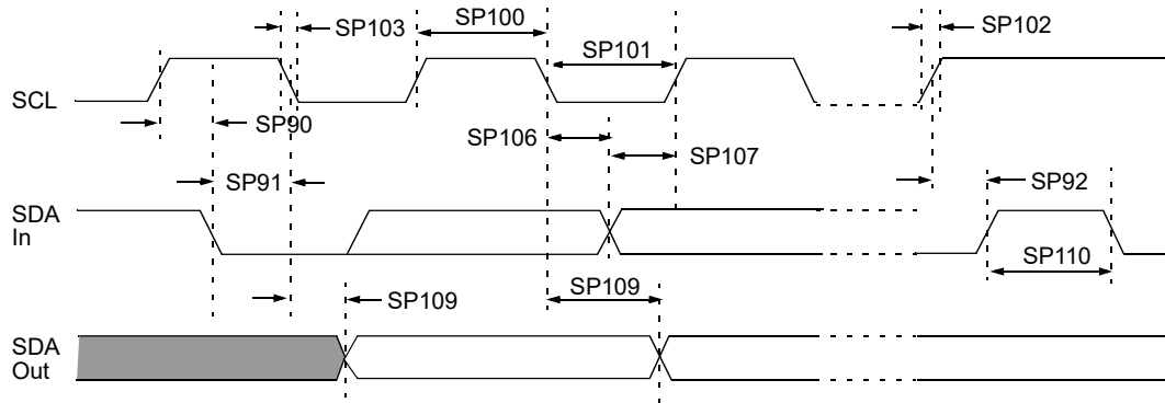
Figure 39-20. I 2 C Bus Data Timing
