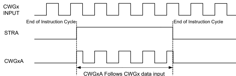
Figure 24-11. Example of Asynchronous Steering ( MODE = 000)
