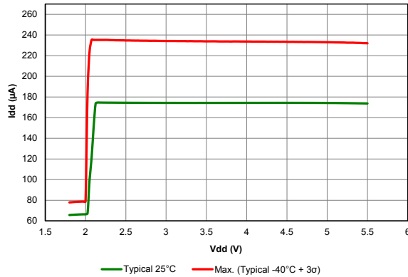
Figure 40-51. I_{PD} BASE (VREGPM='b00)
