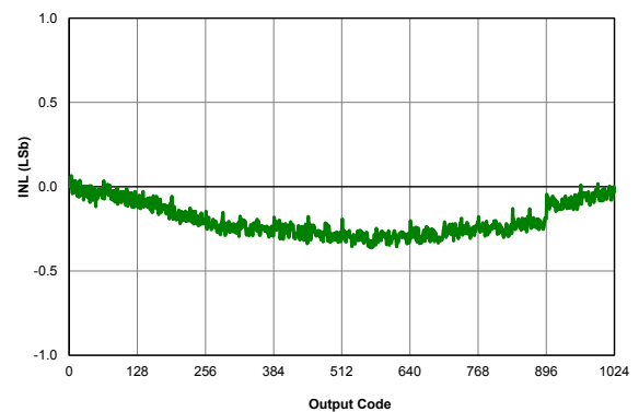
Figure 40-8. ADC 10-BIT, Vdd = 3.0V, VREF = 3.0V, Min and Max values at 125C + 3σ
