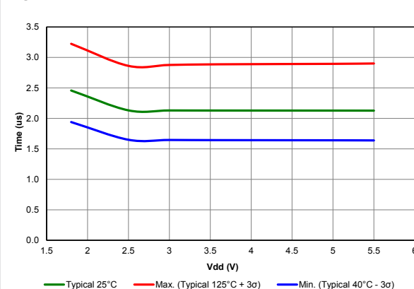
Figure 40-1. ADC RC Oscillator Period vs. Vdd
