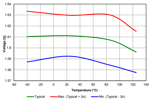
Figure 40-64. POR RELEASE VOLTAGE (VREGPM = 'b1x)
