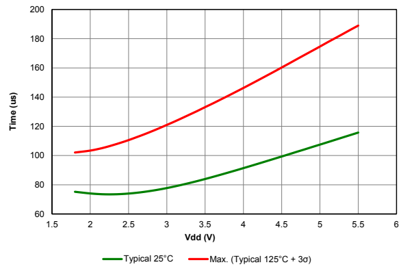
Figure 40-55. Wake From Sleep, VREGPM = 'b10, HFINTOSC = 16MHz
