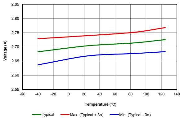
Figure 40-16. BROWN-OUT RESET VOLTAGE, TRIP POINT (BORV = 10)
