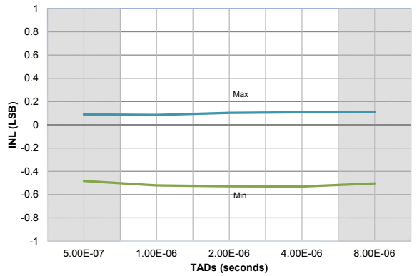
Figure 40-8. ADC 10-BIT, Vdd = 3.0V, VREF = 3.0V, Min and Max values at 125C + 3σ
