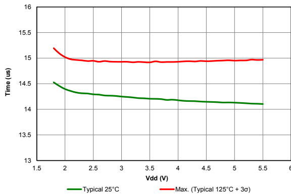
Figure 40-54. Wake From Sleep, VREGPM = 'b0x, HFINTOSC = 16MHz
