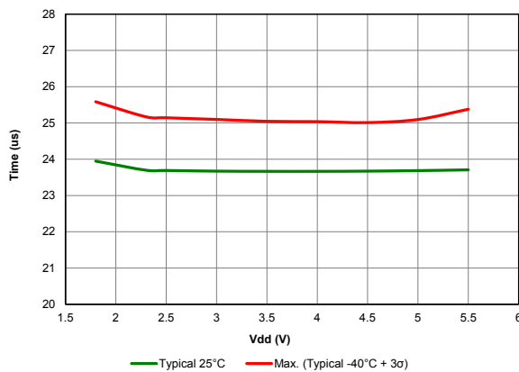
Figure 40-54. Wake From Sleep, VREGPM = 'b0x, HFINTOSC = 16MHz
