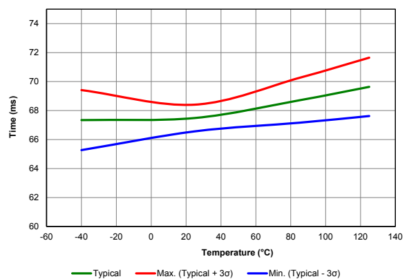
Figure 40-68. PWRT PERIOD vs. Temperature ( V_{DD} = 3.0V )
