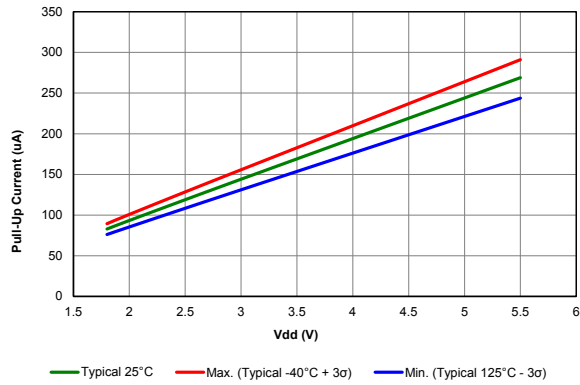
Figure 40-85. Weak Pull-Up Current
