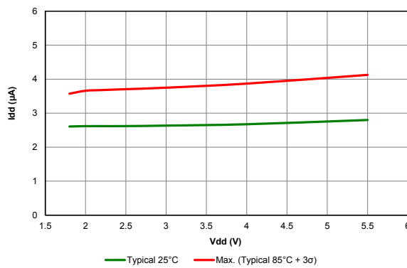
Figure 40-38. I DD MAXIMUM, INT Oscillator
