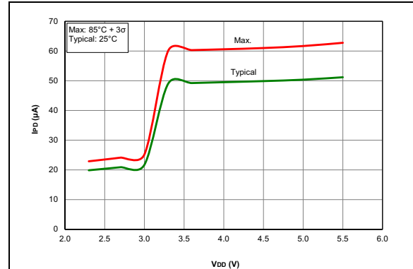
FIGURE 45-52: I PO Base, NP Sleep Mode, PIC18F26/27/45/46/47/55/56/57K42 Only.
