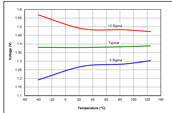
FIGURE 45-138: POR Release Voltage.
