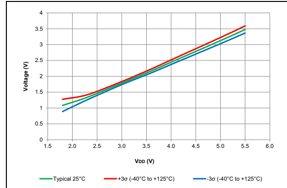
FIGURE 45-130: Schmitt Trigger High Values.
