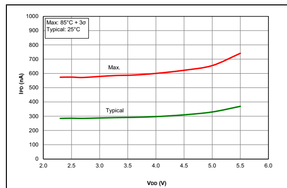
FIGURE 45-53: I PO Base, LP Sleep Mode, PIC18F26/27/45/46/47/55/56/57K42 Only.
