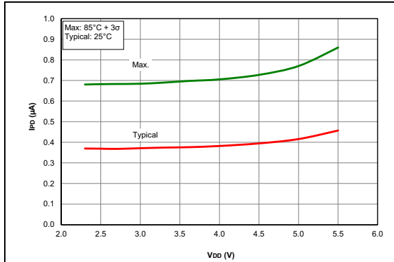
FIGURE 45-49: I PO , Low-Power Brown-Out Reset (LPBOR), PIC18F26/27/45/46/47/55/56/57K42 Only.
