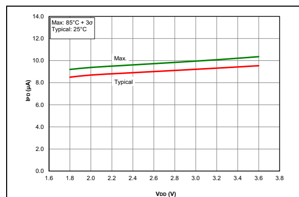
FIGURE 45-54: I PO , High/Low Voltage detect (HLVD), PIC18LF26/27/45/46/47/55/56/57K42 Only.
