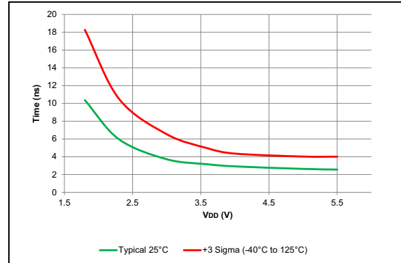
FIGURE 45-136: Fall Time, Slew Rate Control Disabled.
