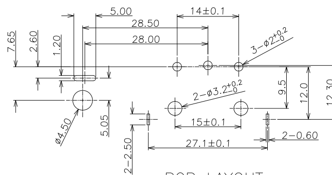
PCB LAYOUT
