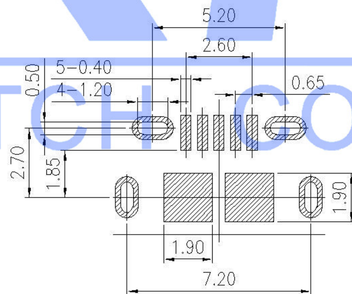
RECOMMENDED PCB LAYOUT(TOP VIEW) GENERAL TOLERANCES:±0.05
