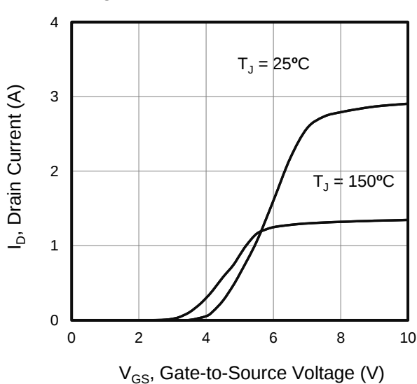
Figure 5. Transfer Characteristics
