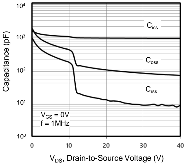
Figure 7. Capacitance
