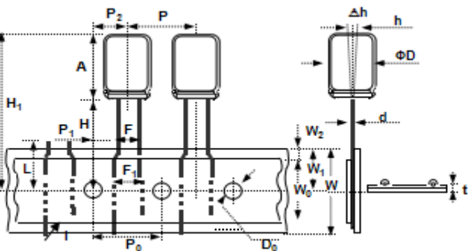
[ Fig. 3 (Diameter for Φ6 to Φ8]
