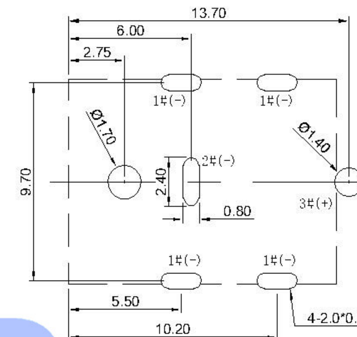
P. C. B LAYOUT
