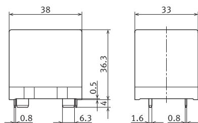
External dimensions
