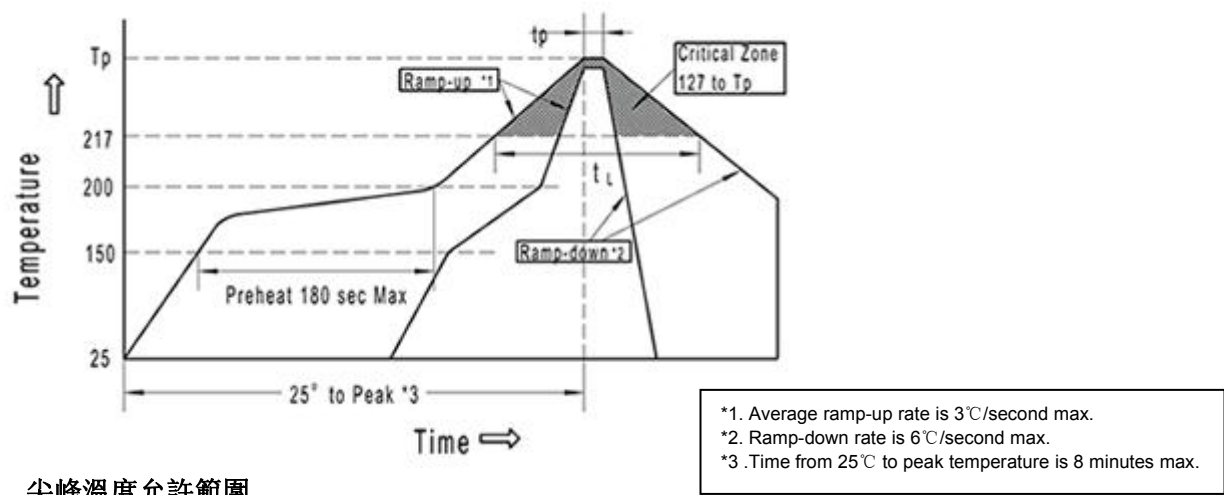
Classification Reflow Profile
