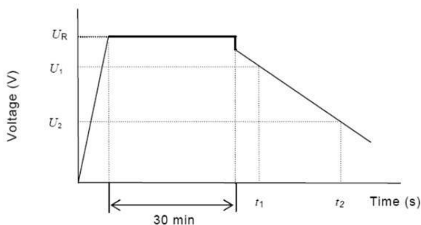
Figure 2 Voltage–time characteristics between capacitor terminals in capacitance measurement
