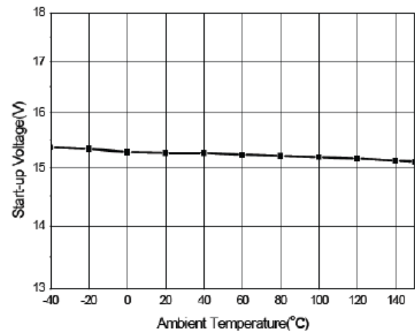
Figure 3. Startup Voltage Vs. Temperature
