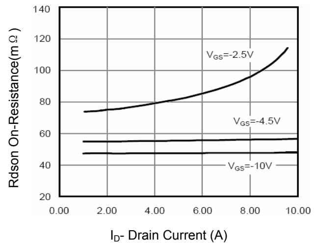
Figure 6 Drain-Source On-Resistance
