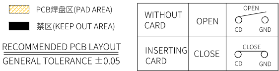
Circuit Diagram for Detect Switch
