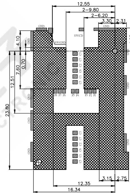
RECOMMENDED PCB LAYOUT(NO PATTERNS) (TOLERANCE: ±0.05) NO PATTERNS
