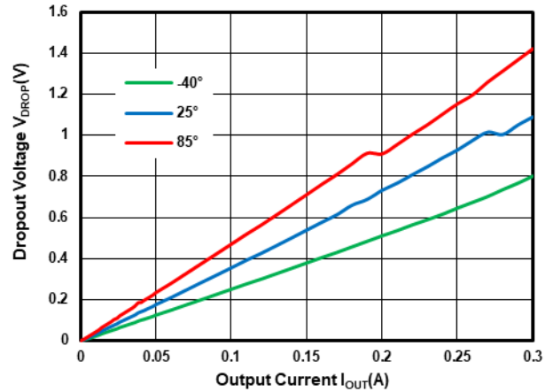
Dropout Voltage vs Temperature at V_{OUT}=3.3V
